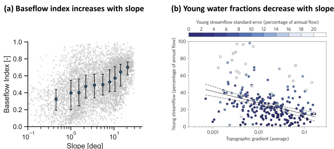
Figure 6. Steeper catchments release more baseflow and older water, as indicated by large samples of catchment data. (a) Baseflow index (BFI; the ratio of baseflow to total streamflow) against topographic slope (Spearman rank correlation \rho_s = 0.44 ) for 6,830 catchments from the Caravan data set (Kratzert et al., 2023a). Note that accounting for aridity (partial \rho_s = 0.44 ) and snow fraction (partial \rho_s = 0.42 ) via partial correlations does not alter the correlation substantially. (b) Young water fractions against topographic slope ( \rho_s = -0.36 ), taken from Jasechko et al. (2016) with permission from Springer Nature.
