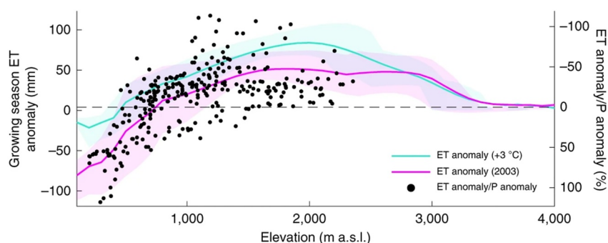
Figure 3. Drought paradox in the European Alps. During the 2003 heatwave or with a warming climate, actual evaporation will respond differently with elevation. At low elevations, water is limited and evaporation is reduced, while at high elevations greater evaporative demand and longer growing seasons enhance evaporation. The solid lines (left axis) show evaporation anomalies, computed based on the 2001–2003 mean and averaged over 100 m elevation bins, for the 2003 heatwave (magenta) and for a +3°C climate change scenario (cyan); the shaded areas show interquartiles ranges. The solid points (right axis) show the ratio of evaporation anomalies to precipitation anomalies for 334 catchments, indicating how strongly evaporation anomalies contributed to the streamflow deficits during the 2003 growing season. From Mastrotheodoros et al. (2020) with permission from Springer Nature.
